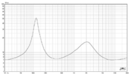
Impedance Graph:
